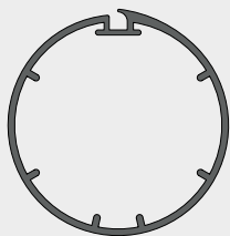
Rullo standard diametro 43 mm Ø interno 40,90 mm Ø esterno 43,39 mm
